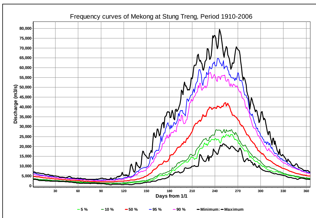
Figure 4-2 Frequency curves of the Mekong River discharge at Stung Treng, period 1910-2006.
