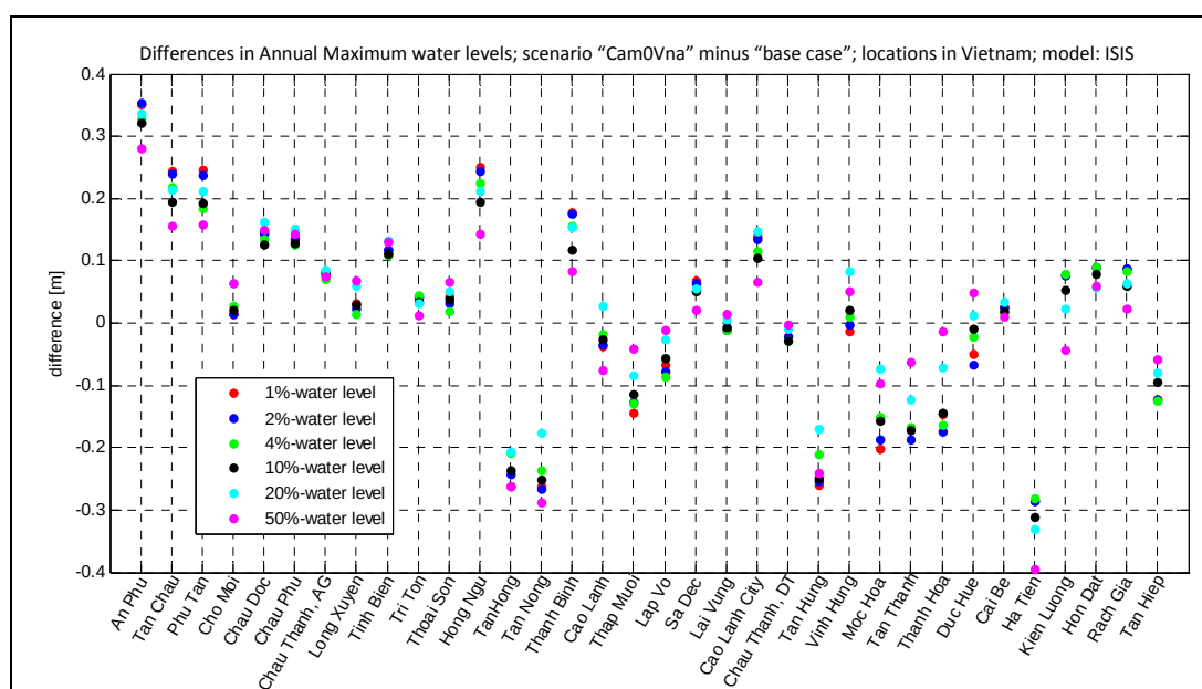
Figure 5-23 Change in the p-percent annual maximum water level (p=1, 2, 4, 10, 20 and 50) for 34 locations in Vietnam; comparison of scenario Cam0VNa with the Base Case. Positive values indicate an increase in water level.
