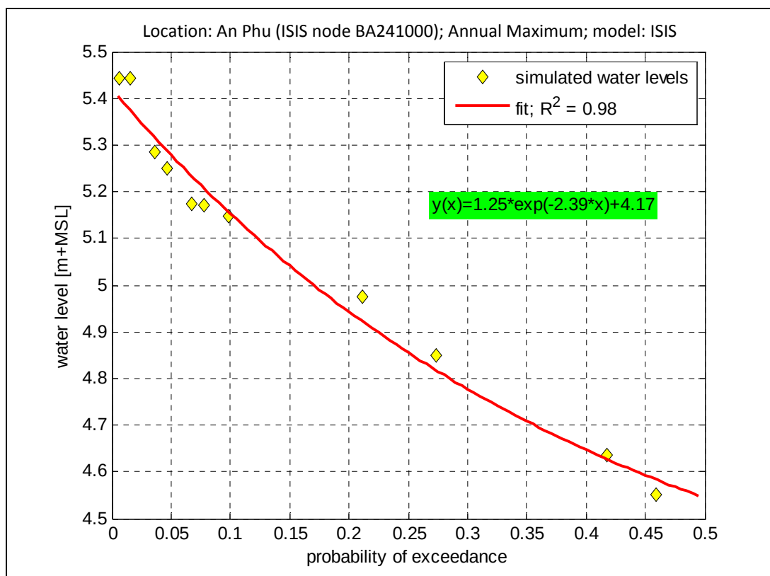
Figure 5-6 Fitted function of probability of exceedance for water levels for location An Phu; Base Case.
