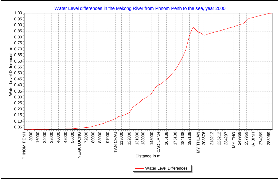
Figure 5-37 Net effect of 1 m sea level rise on the maximum water level in Mekong, conditions of year 2000.
