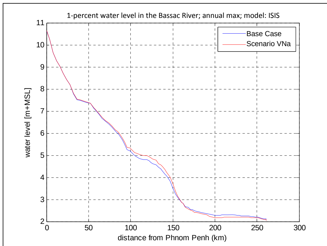
Figure 5-20 Water levels in the Bassac River downstream of Phnom Penh; comparison between the Base Case and scenario VNa.
