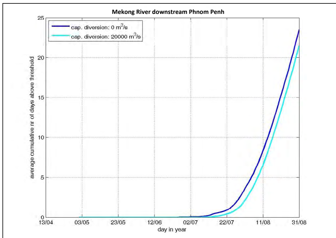
Figure 5-31 Average cumulative number of days (up to the date shown on the horizontal axis) in the simulated period 1910-2006 during which the flow downstream of Phnom Penh exceeded 30,000 m 3 /s; depending on the available flow capacity of the diversion channel.
