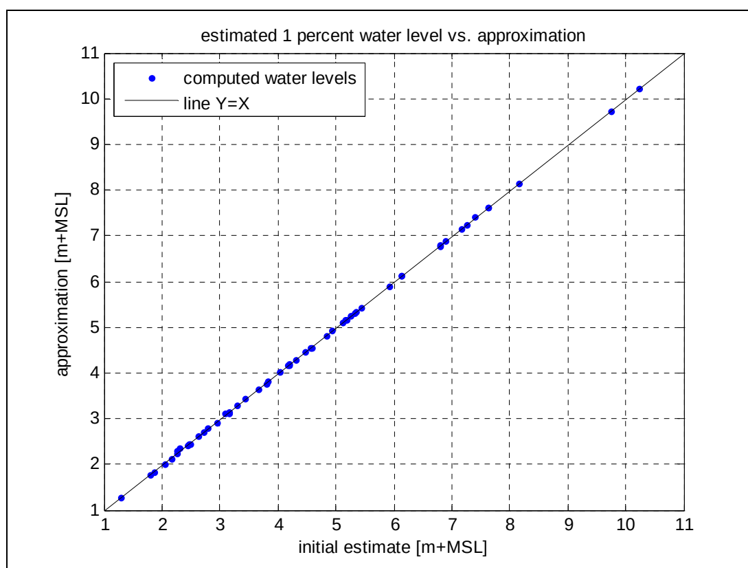
Figure 5-9 Comparison of the estimated 1%-water level (i.e. the 100 year water level) based on 97 simulated years (horizontal axis) and the approximated estimate based on 11 simulated years (vertical axis). The comparison is made for the 59 selected locations.
