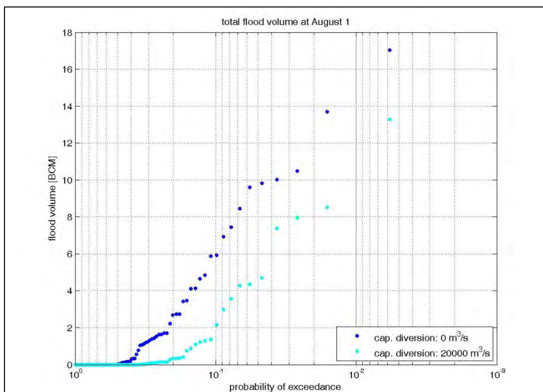
Figure 5-32 Frequency distribution of the total volume above a threshold of 30,000 m 3 /s in the Mekong River downstream of Phnom Penh until August 1, depending on the available flow capacity of the diversion channel.
