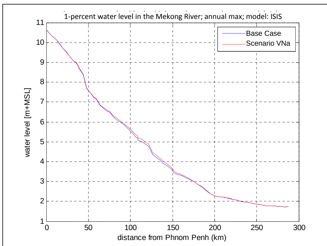
Figure 5-18 Water levels in the Mekong River downstream of Phnom Penh; comparison between the Base Case and scenario VNa.
