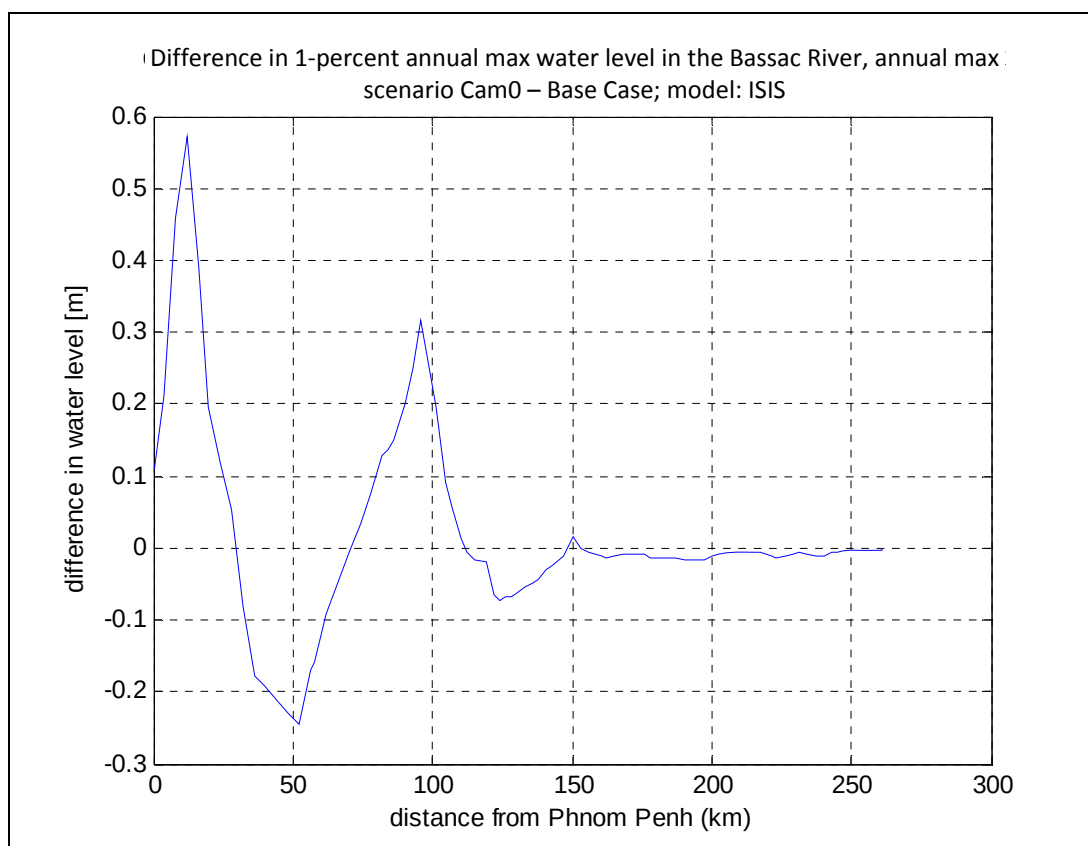
Figure 5-15 Increase in water level in the Bassac River downstream of Phnom Penh as a result of scenario Cam0 (differences between the two cases of Figure 5-14).
