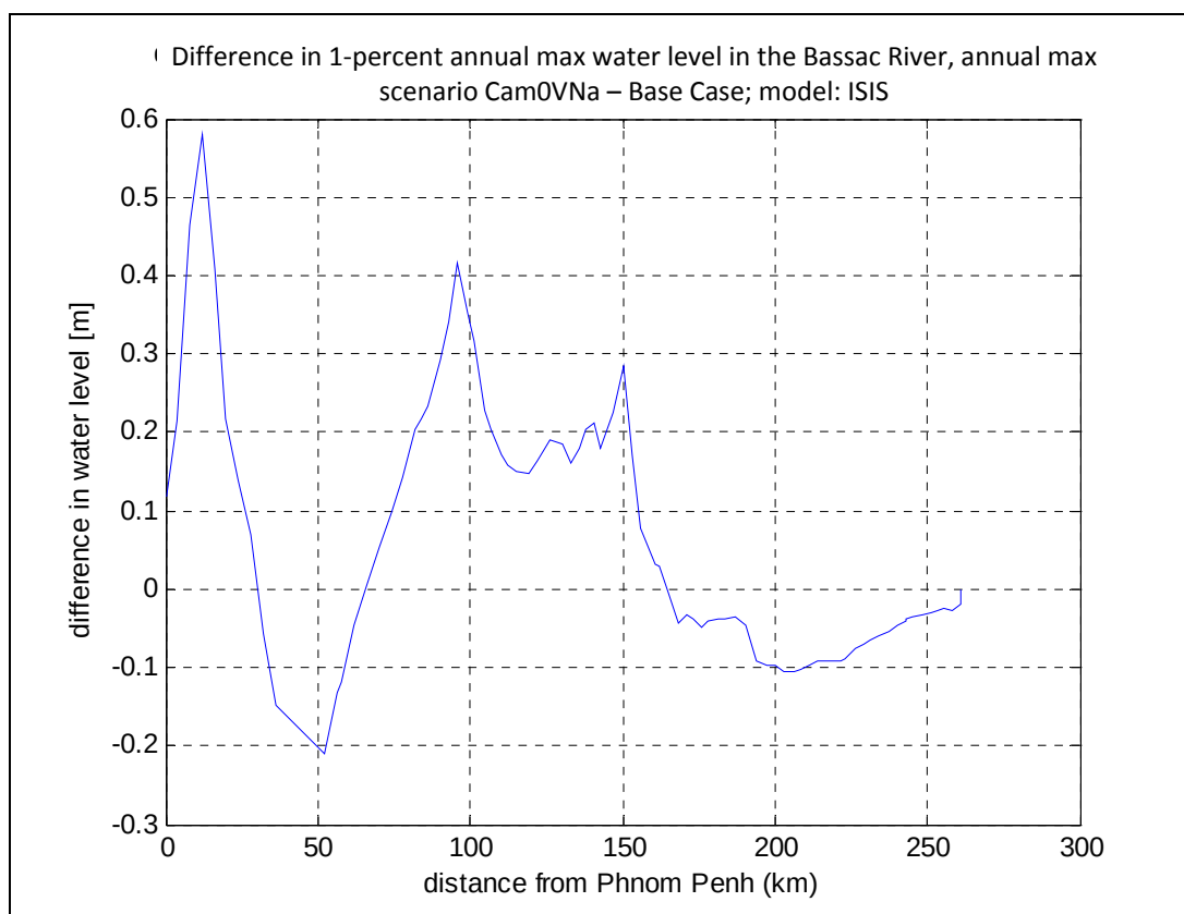
Figure 5-27 Increase in water level in the Bassac River downstream of Phnom Penh as a result of scenario Cam0VNa.
