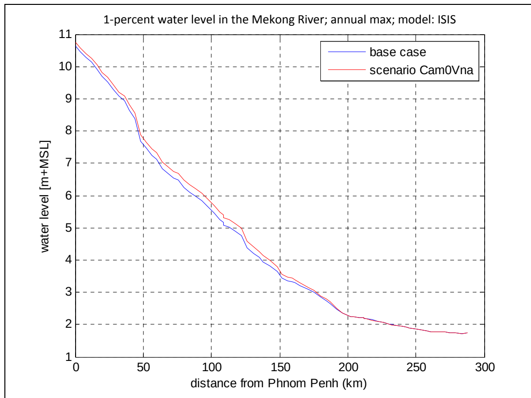
Figure 5-24 Water levels in the Mekong River downstream of Phnom Penh; comparison between the Base Case and scenario Cam0VNa.
