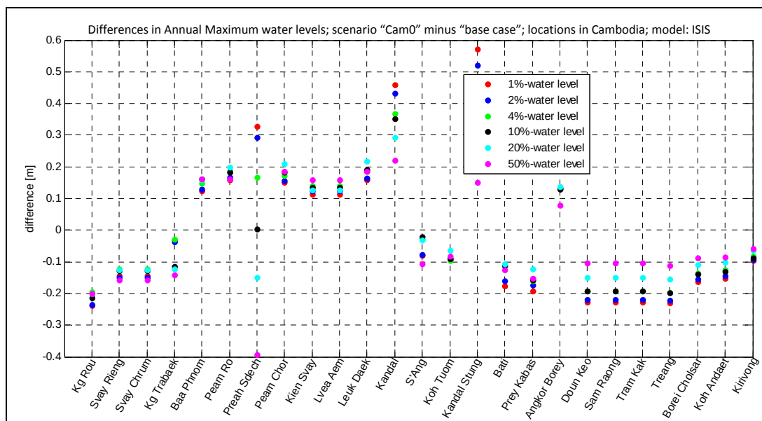
Figure 5-10 Change in the p-percent annual maximum water level (p=1, 2, 4, 10, 20 and 50) for 25 locations in Cambodia; comparison of scenario Cam0 with the Base Case. Positive values indicate an increase in water level.
