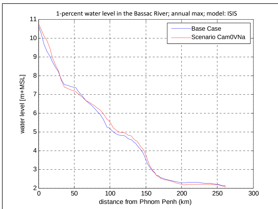
Figure 5-26 Water levels in the Bassac River downstream of Phnom Penh; comparison between the Base Case and scenario Cam0VNa.
