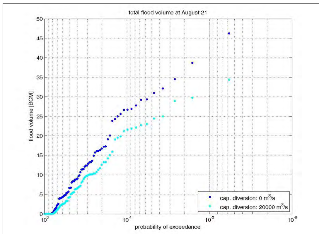
Figure 5-33 Frequency distribution of the total volume above a threshold of 30,000 m 3 /s in the Mekong River downstream of Phnom Penh until August 21, depending on the available flow capacity of the diversion channel.
