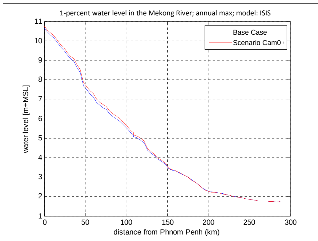
Figure 5-12 Water levels in the Mekong River downstream of Phnom Penh; comparison between the Base Case and scenario Cam0.
