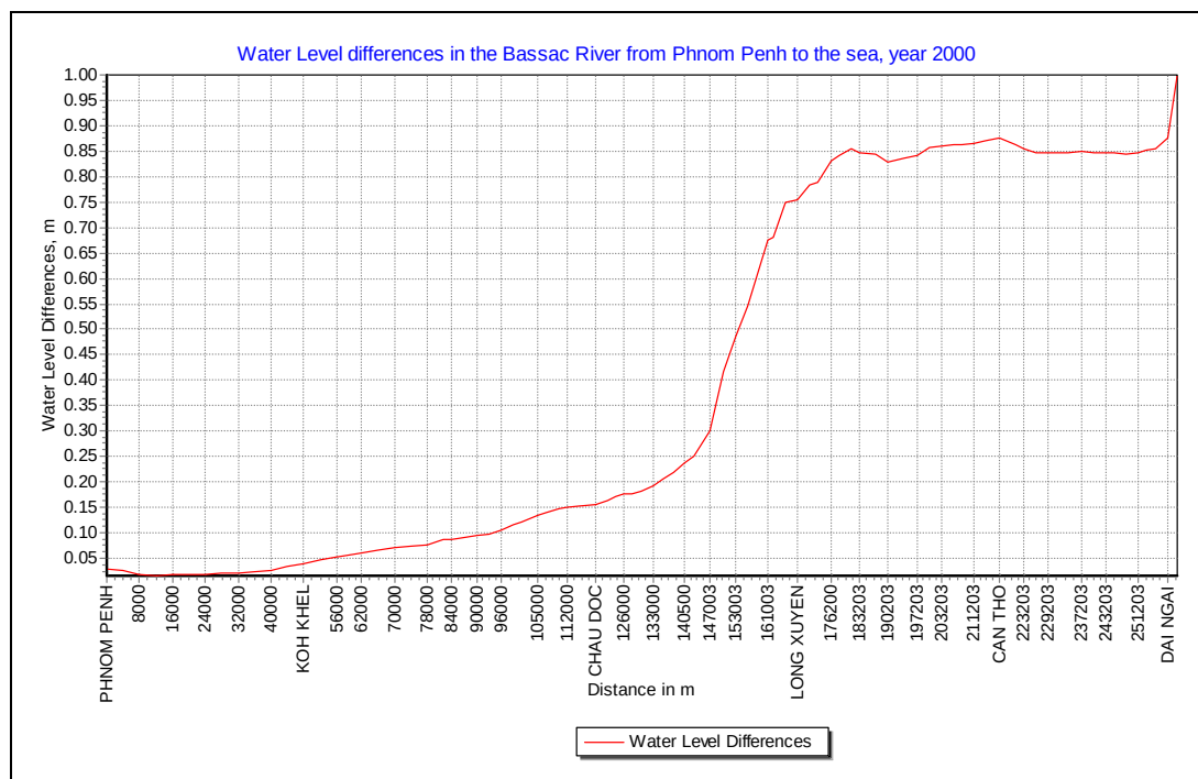
Figure 5-35 Net effect of 1 m sea level rise on the maximum water levels in Bassac, conditions of year 2000.
