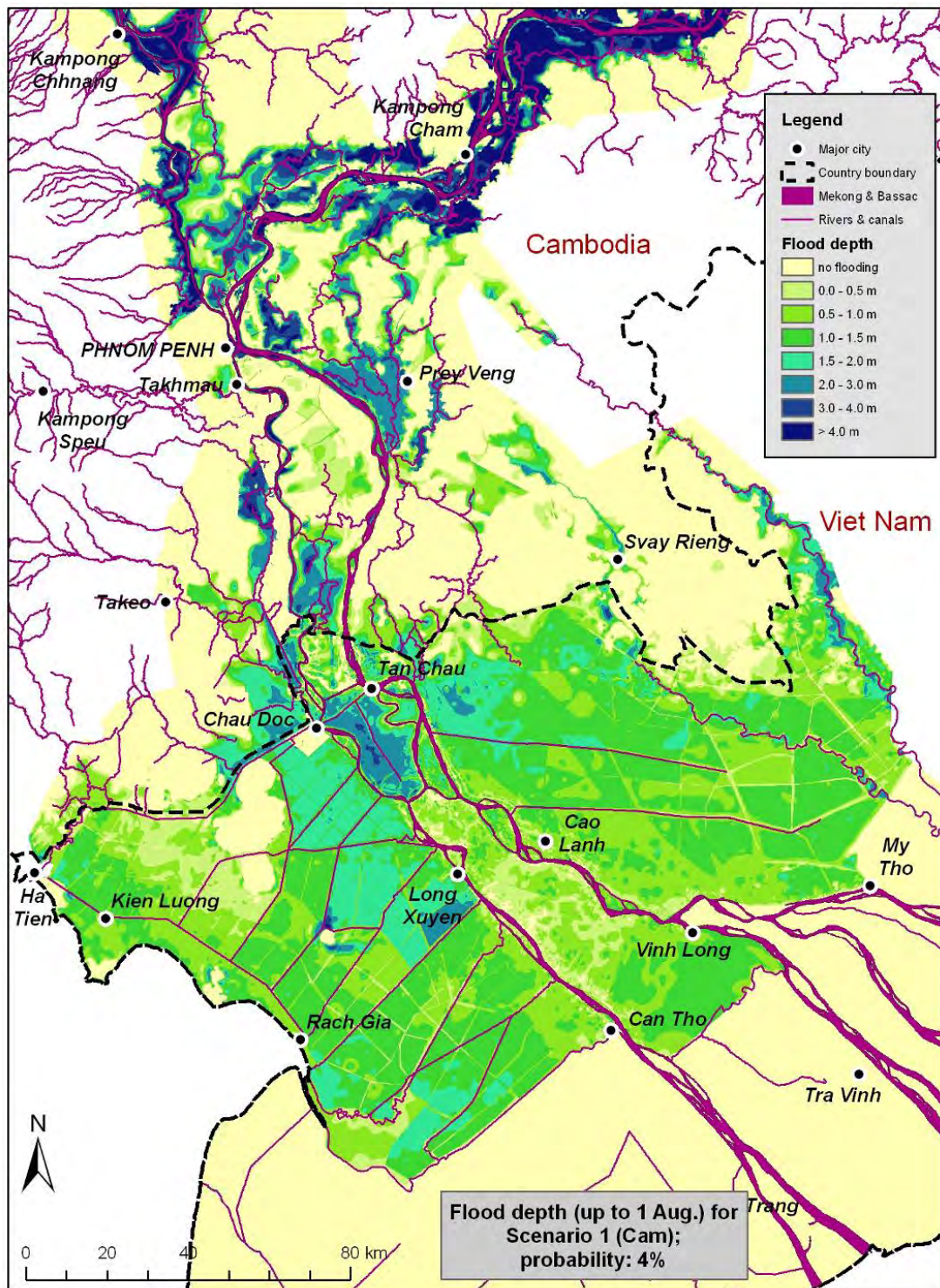
Attachment 1.1.12 Flood Hazard map at p=4%, Scenario Cam0, before 1st of August
