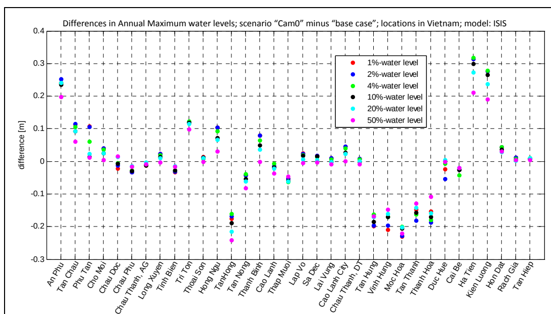
Figure 5-11 Change in the p-percent annual maximum water level (p=1, 2, 4, 10, 20 and 50) for 34 locations in Vietnam; comparison of scenario Cam0 with the Base Case. Positive values indicate an increase in water level.
