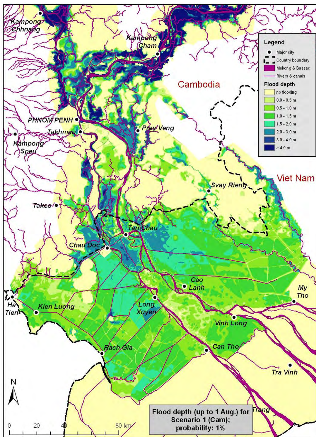
Attachment 1.1.11 Flood Hazard map at p=1%, Scenario Cam0, before 1st of August
