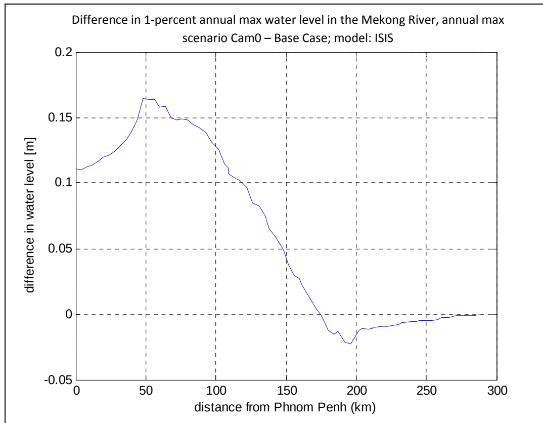
Figure 5-13 Increase in water level in the Mekong River downstream of Phnom Penh as a result of scenario Cam0 (differences between the two cases of Figure 5-12).
