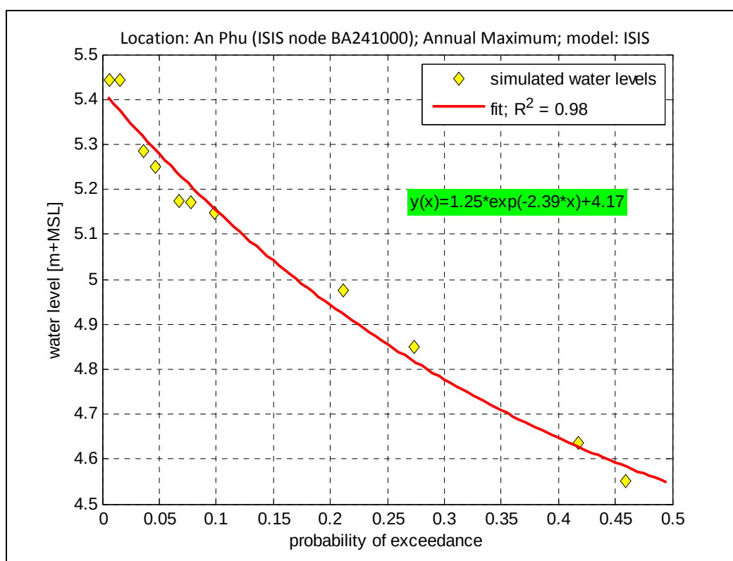
Figure 5-8 Fitted function of probability of exceedance for water levels for location An Phu; scenario Cam0.
