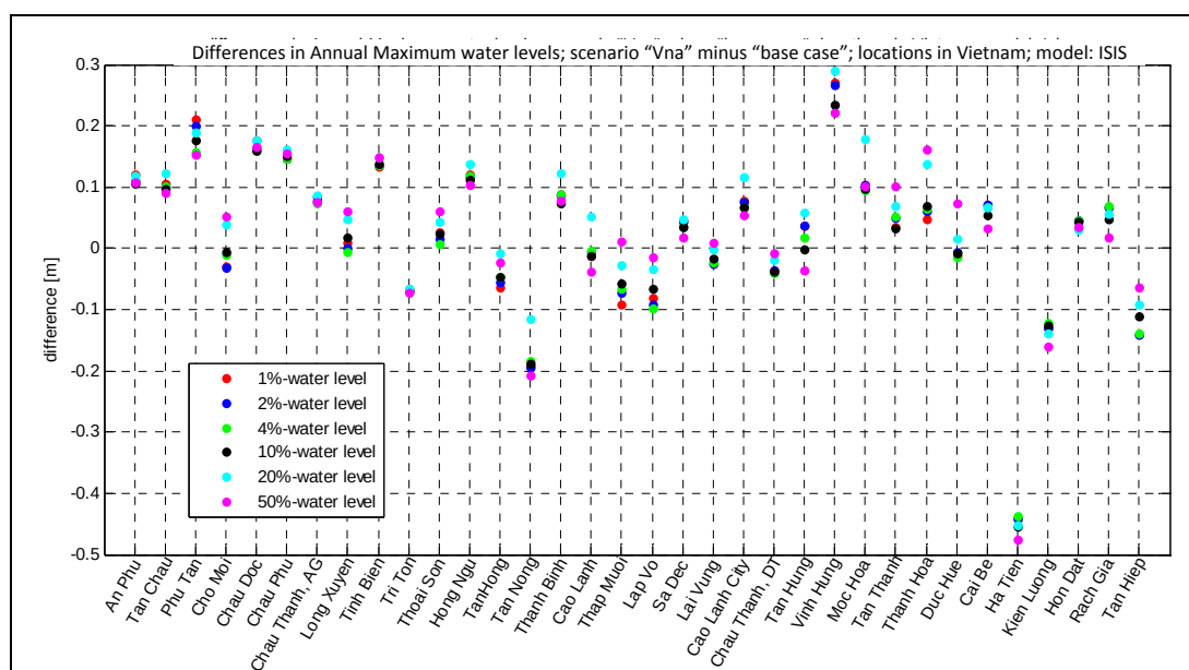
Figure 5-17 Change in the p-percent annual maximum water level (p=1, 2, 4, 10, 20 and 50) for 34 locations in Viet Nam; comparison of scenario VNa with the Base Case. Positive values indicate an increase in water level.
