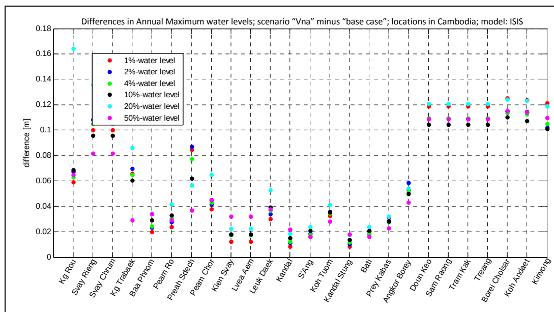
Figure 5-16 Change in the p-percent annual maximum water level (p=1, 2, 4, 10, 20 and 50) for 25 locations in Cambodia; comparison of scenario VNa with the Base Case. Positive values indicate an increase in water level.
