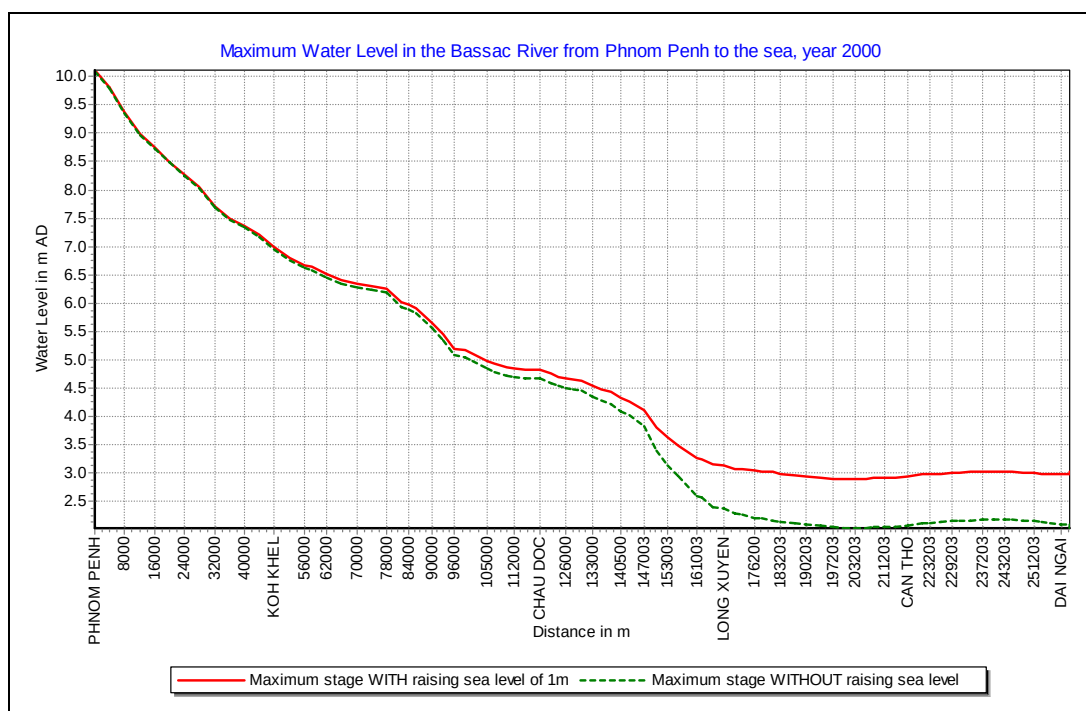
Figure 5-34 Effect of 1 m sea level rise on the maximum water level in Bassac, conditions of year 2000.
