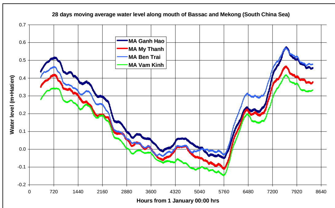
Figure 3-9 28 days moving average of water level at Ganh Hao, My Thanh, Ben Trai and Vam Kinh.
