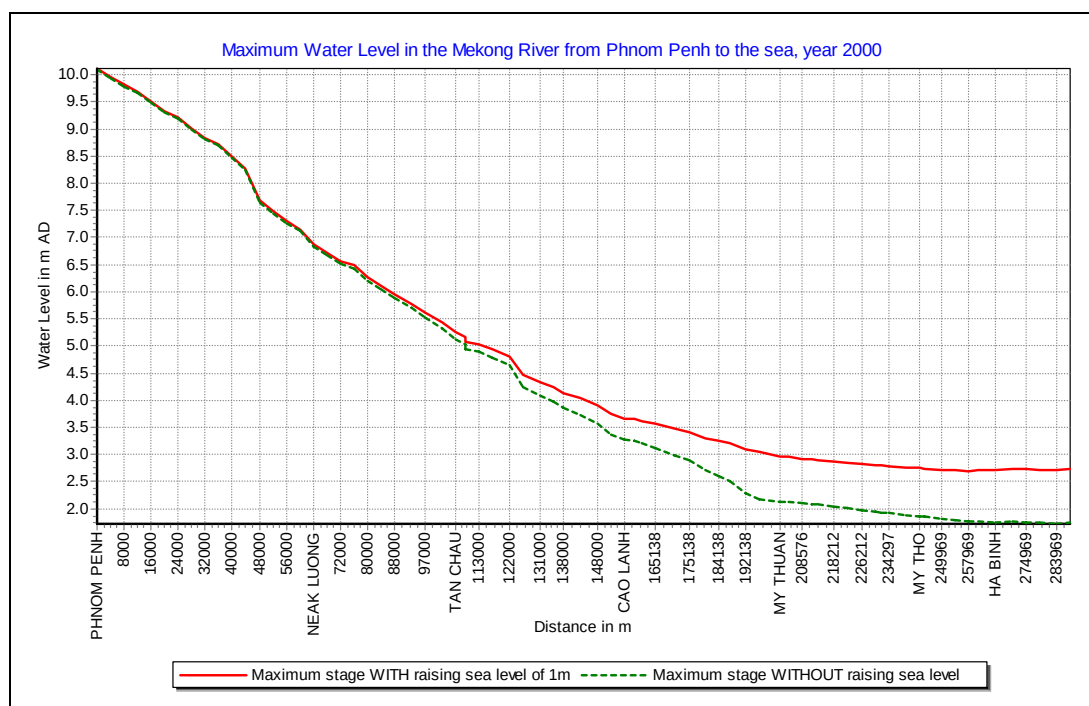
Figure 5-36 Effect of 1 m sea level rise on the maximum water level in Mekong, conditions of year 2000.
