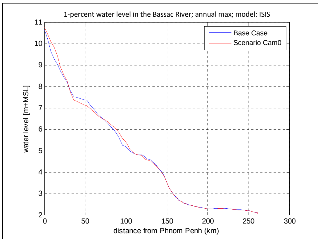
Figure 5-14 Water levels in the Bassac River downstream of Phnom Penh; comparison between the Base Case and scenario Cam0.
