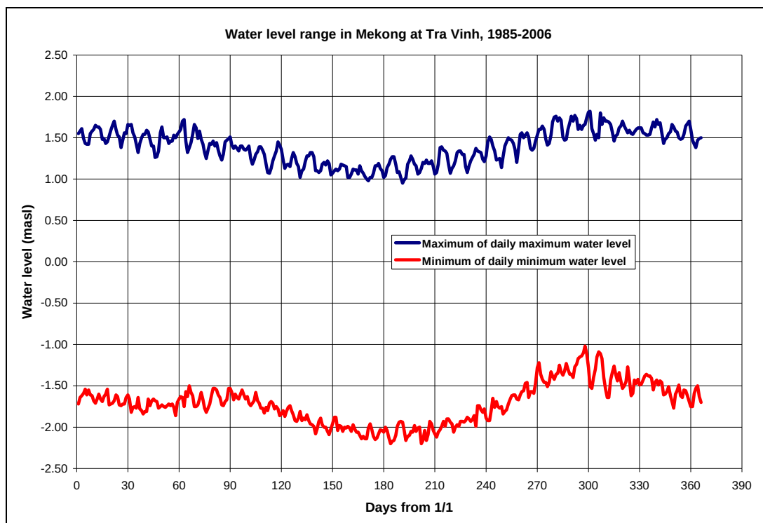
Figure 3-8 Water level range in Mekong River at Tra Vinh near the coast, period 1985-2006.
