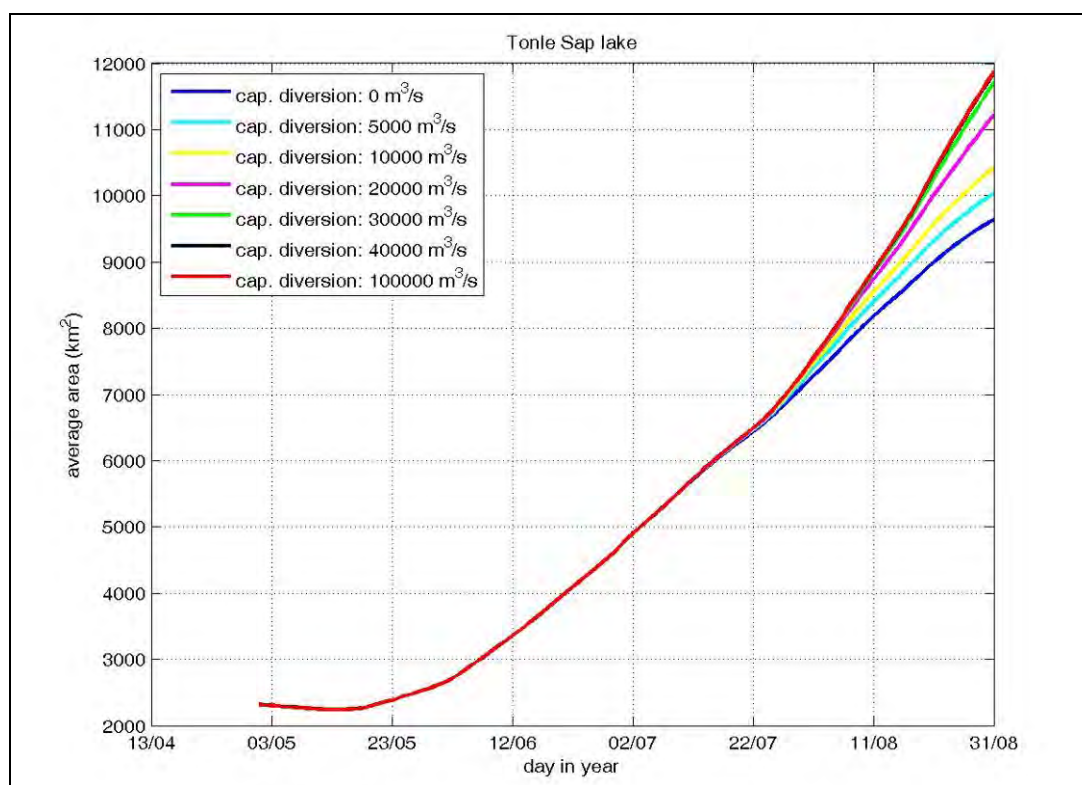
Figure 5-30 Mean wet surface area of the lake for different values of the flow capacity of the diversion.
