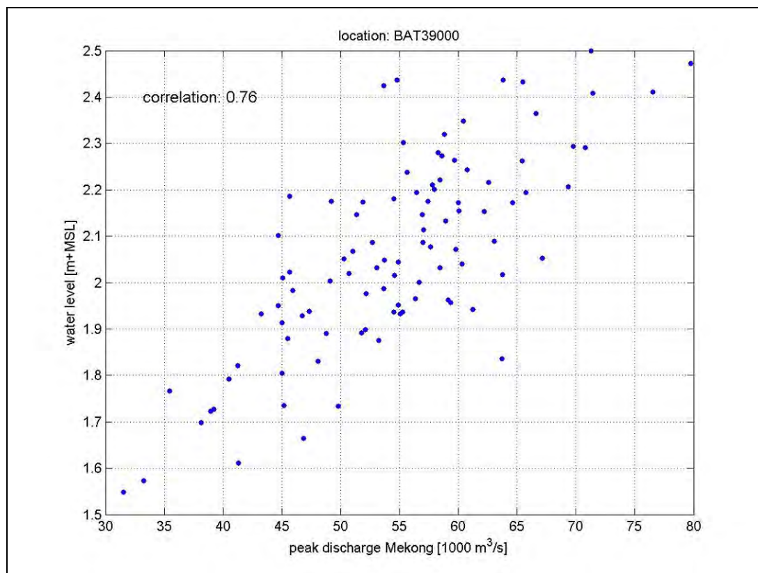
Figure 5-5 Annual peak discharges (1000 m 3 /s) in the Mekong River at Stung Treng versus annual maximum water level at model node BAT39000.
