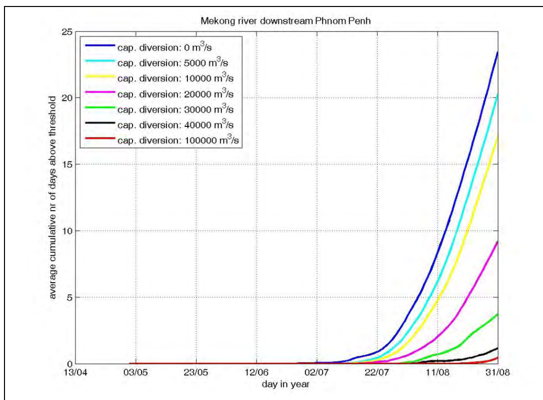
Figure 5-29 Average cumulative number of days (up to the date shown on the horizontal axis) in the simulated period 1910-2006 during which the flow downstream of Phnom Penh exceeded 30,000 m 3 /s; depending on the available flow capacity of the diversion channel.
