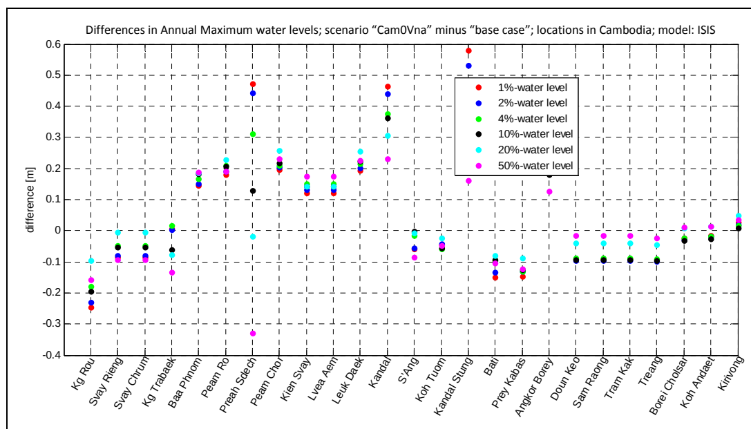
Figure 5-22 Change in the p-percent annual maximum water level (p=1, 2, 4, 10, 20 and 50) for 25 locations in Cambodia; comparison of scenario Cam0VNa with the Base Case. Positive values indicate an increase in water level.
