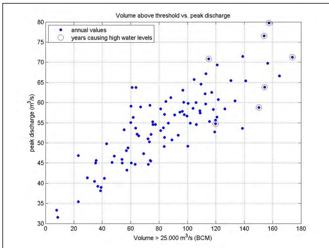
Figure 5-3 Volume of flow above the threshold of 25.000 m³/s versus peak discharge.
