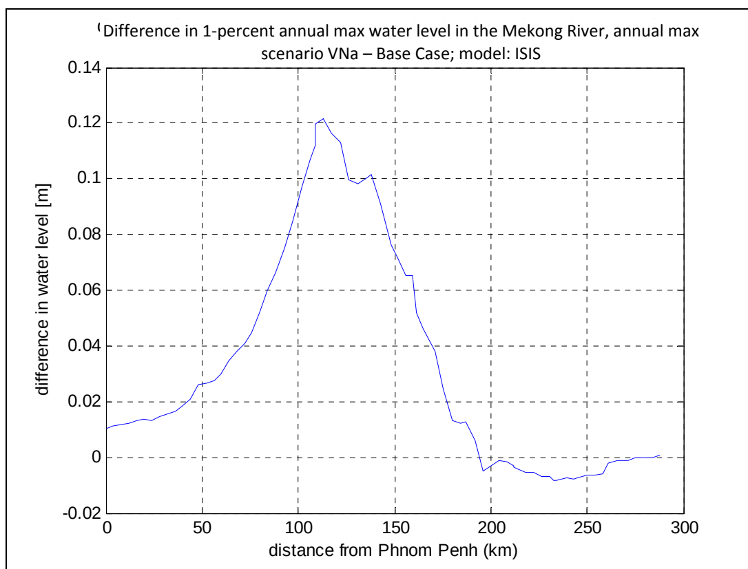
Figure 5-19 Increase in water level in the Mekong River downstream of Phnom Penh as a result of scenario VNa.
