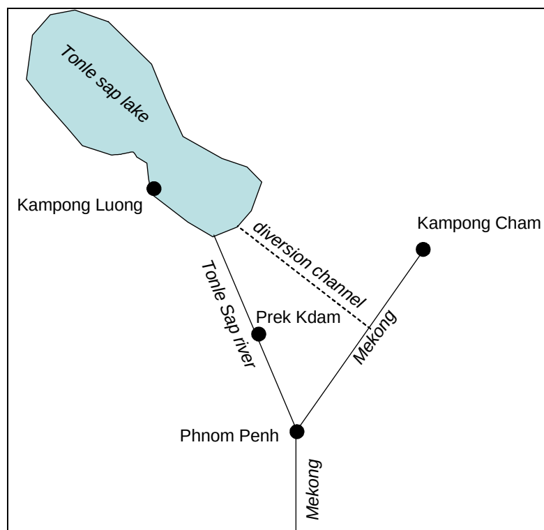
Figure 5-28 Structure of water balance model of Mekong River and Tonle Sap.
