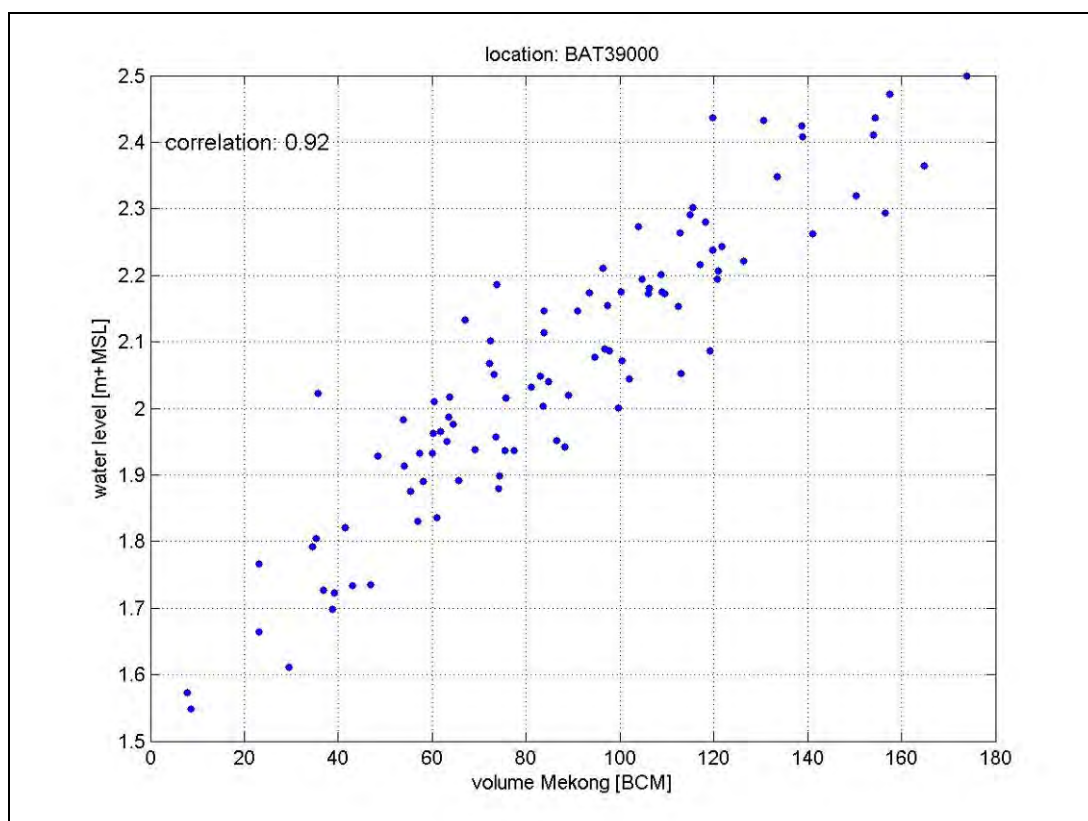
Figure 5-4 Annual flow volumes (BCM) in the Mekong River at Stung Treng above a threshold discharge of 25,000 m³/s versus annual maximum water level at model node BAT39000.
